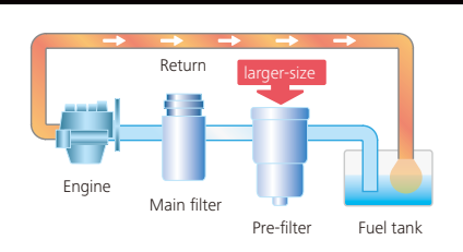
Recognized as the best in the industry, our Premium-fine filter separates out even the smallest particles. New cover prevents contamination when changing filters.
