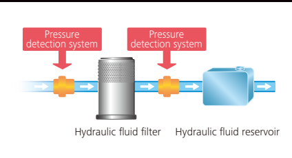
Hydraulic tank pressure sensor monitors the pressure difference between the return line and tank inside pressure to determine the degree of clogging. If the difference exceeds a predetermined level, a warning appears on the multi-display, so any contamination can be trapped by the filter and replaced before it reaches the hydraulic fluid in the tank.
